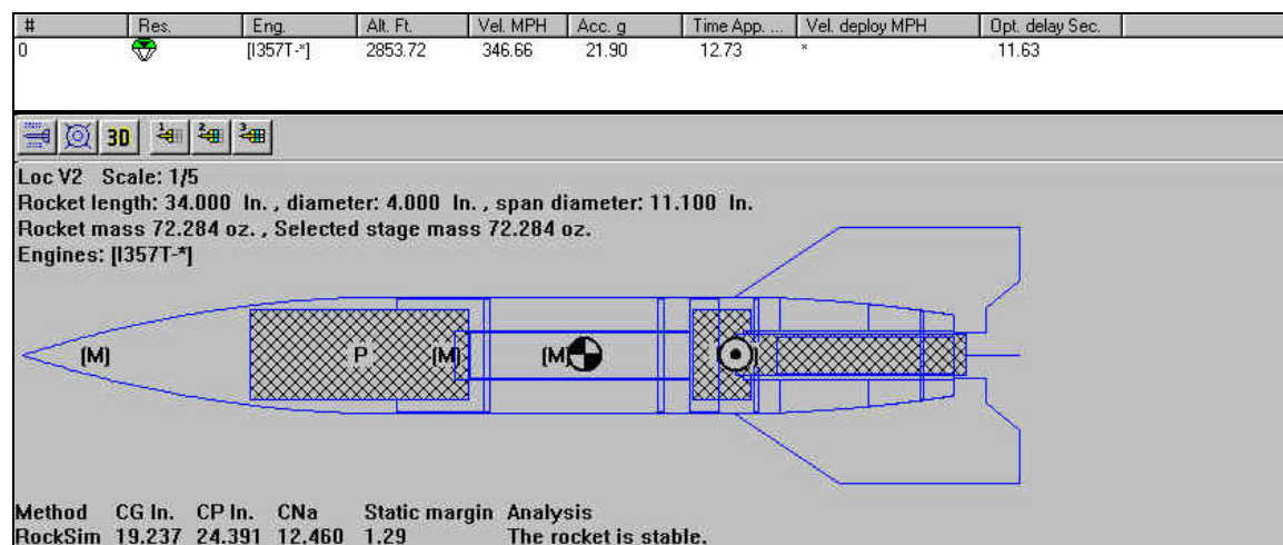
Figure 5: RockSim Simulation
